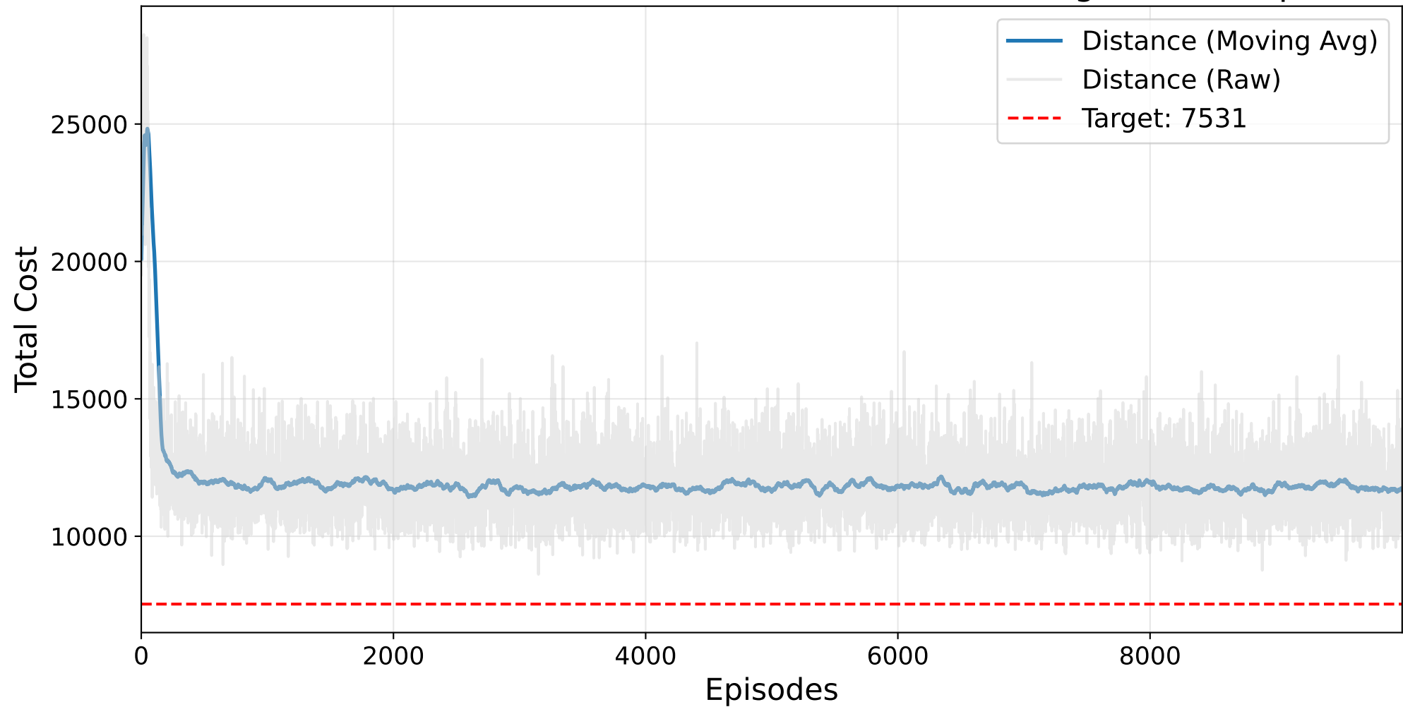
Final HYPERBAND GP Masked AutoRL-SOP Training - ft53.1.sop
